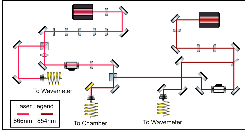
Figure 5.10: Calcium repumps (854 nm + 866 nm) beampath (on table).
