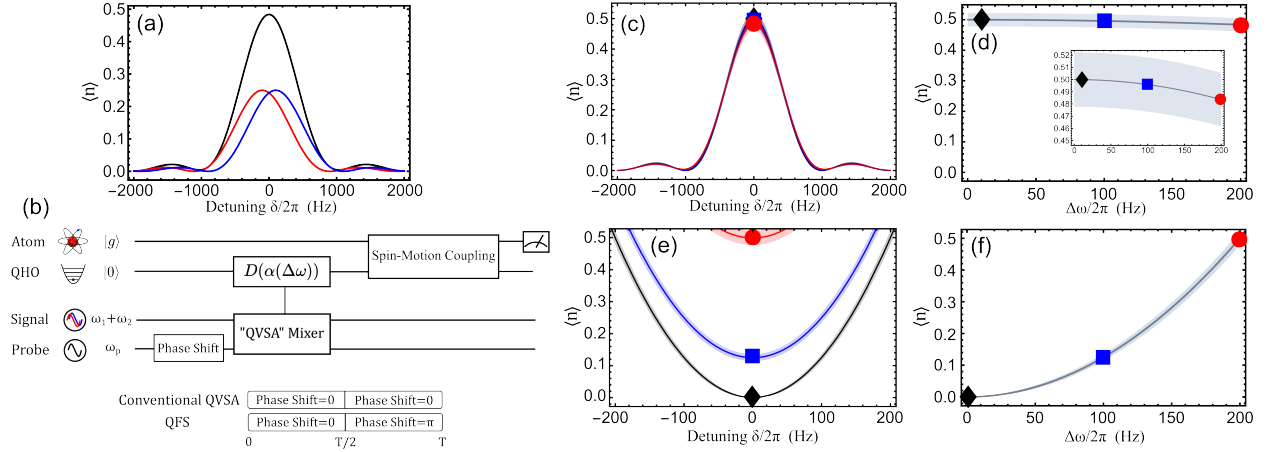
Figure 10.1: Spectroscopy of two incoherent tones using conventional Quantum Vector Signal Analyzer/Analysis (QVSA) and Quantum Fluctuation Suppression (QFS) techniques. (a) Conventional spectroscopy with two incoherent signal tones. When the separation between the two tones falls below the traditional linewidth limit, their corresponding peaks (red and blue traces) merge (black trace) and become unresolvable. (b) Quantum circuits implementing conventional QVSA and QFS protocols for detecting the frequency difference \Delta\omega = \omega_2 - \omega_1 . The QFS protocol is implemented by applying a \pi phase shift to the probe tone at time T/2 . The “QVSA” mixer is realized by a motional Raman transition and heterodynes the quadrupolar probe and unknown signal tones, resulting in a displacement of the Quantum Harmonic Oscillator (QHO) [Wu+25b]. Expected (c) conventional and (e) QFS spectroscopy generated by scanning the probe detuning ( \delta ) at several different \Delta\omega . (c, d, e, f) Expected mean phonon number \langle n \rangle under the conventional protocol (d) and the QFS protocol (f) as a function of \Delta\omega at zero detuning \delta = 0 . Shaded regions represent the uncertainty \sigma_{\langle n \rangle} due to phonon shot noise for N = 1000 trials. (d) Using the conventional protocol, the dominant source of shot noise in the measured \langle n \rangle is independent of \Delta\omega , obscuring any dependence of \langle n \rangle on \Delta\omega and rendering \Delta\omega unresolvable. (f) Using the QFS protocol, sensitivity to \Delta\omega is recovered by nullifying the \Delta\omega -independent shot noise at \delta = 0 . Here, the interrogation time is T = 1 ms.
