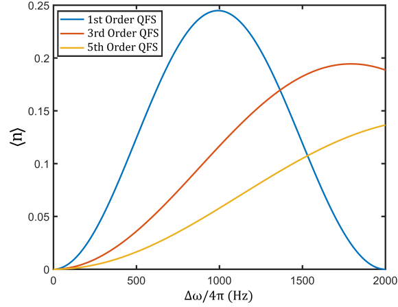
Figure 10.10: Resultant mean phonon number \langle n \rangle calculated as a function of the signal frequency separation \Delta\omega using higher protocol orders (i.e. number of phase reversals). Only odd QFS orders are shown as only these achieve full suppression of \Delta\omega -independent background. All curves have been calculated using identical parameters ( \Omega_{\text{eff}} , T = 1 ms).
