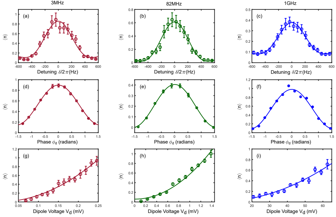
Figure 8.7: Wideband demonstration of frequency, phase, and amplitude sensing using the QVSA. (a)-(c) Dipole signals are detected by sweeping a pair of quadrupole tones across \omega_d/2\pi = 3 MHz, 82 MHz, and 1 GHz, respectively. The lineshape \langle n \rangle = |\alpha|^2 is obtained by varying the detuning \delta . (d)-(f) illustrate the dependence of \langle n \rangle on \phi_d for 3 MHz, 82 MHz, and 1 GHz, respectively. The phase dependence is measured with detuning \delta = 0 . The quadratic dependence of \langle n \rangle on V_d is measured in (g)-(i). The combination of frequency, phase, and amplitude sensing provide the means for vector signal analysis. Solid lines are fit using eq. (8.2) to extract the voltages experienced by the ion. Error bars represent one standard error. Exact parameters used for each panel are listed in Table 8.1.
