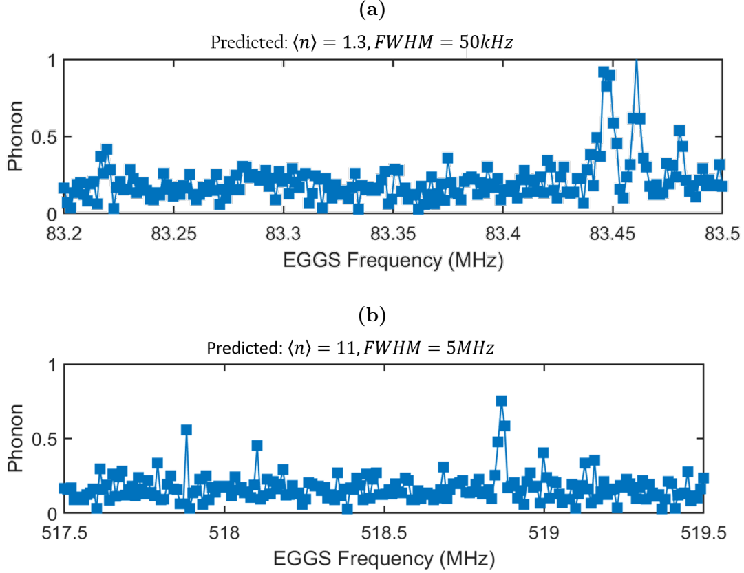
Figure 7.12: Peak data from the EGGS QLS search.
