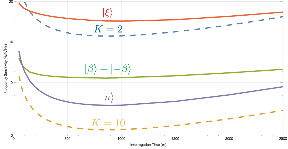
Figure 9.10: Simulated frequency sensitivity using a motional Ramsey protocol (displace - delay - antidisplace) with different amplification strategies in the presence of dephasing ( T_2 = 2 ms). The amplification-free case is represented by the |K = 2\rangle linear protocol, which uses |\alpha = 0.1\rangle . Quantum amplification with nonclassical states is implemented by applying this K = 2 , |\alpha = 0.1\rangle linear protocol to the nonclassical state, then time-reversing the nonclassical dynamics. We simulate quantum amplification of the motional Ramsey using a Fock state ( |n\rangle , n = 5 ), a squeezed state ( |\xi\rangle , \xi = 1.544 ), and a cat state ( |\beta\rangle + |-\beta\rangle , \beta = 2.236 ). The parameters of the nonclassical states have been chosen to keep the mean phonon number \bar{n} = 5 . Amplification with our nonlinear protocol is implemented by instead generating the displacement of the motional Ramsey using a higher-order subharmonic, shown here as the K = 10 subharmonic. For fair comparison, the displacement is kept the same as that with the nonclassical protocols, i.e. \alpha = 0.1 .
