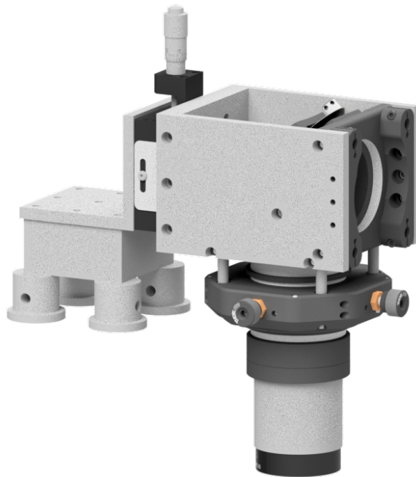
Figure 5.7: Imaging assembly for the objective lens.
