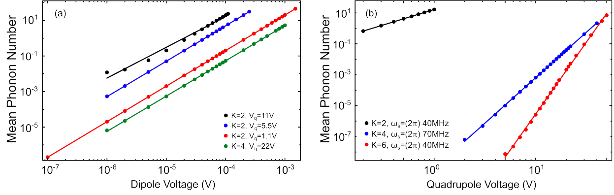
Figure 9.2: Dependence of the subharmonic excitation on the applied dipole voltage V_d and the applied quadrupole voltages V_s, V_q , respectively. Results are simulated using a \omega = 1 MHz secular frequency. A linear model y = mx + b is fitted to the log-log transform of the results to extract the power-law dependence at each subharmonic order. (a) Simulated results at all subharmonic orders exhibit an approximately quadratic dependence of mean phonon number on dipole voltage V_d , equivalent to a linear dependence of displacement on V_d . \omega_s/2\pi = 40 MHz. (b) Simulated results exhibit a power-law scaling of the mean phonon number on V_q , using a V_d = 1 mV, that agrees well with the predicted scaling of 2(K - 1) .
