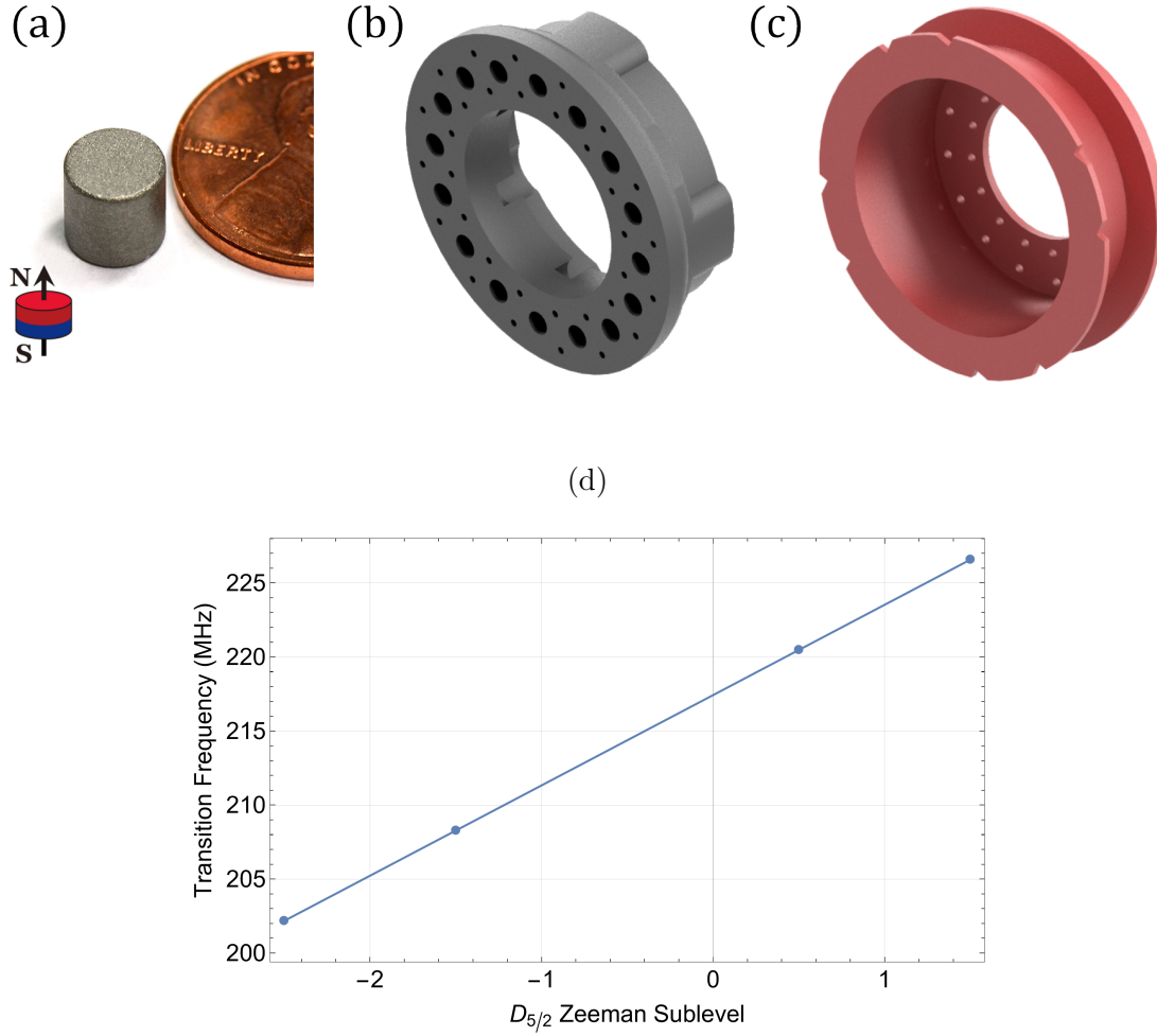
Figure 5.6: Magnetic field apparatus used to define the quantization axis. (a, b) SmCo magnets (US penny for scale) are mounted into 3D-printed holders that arrange the magnets into arrays to generate the quantization field. (c) 3D-printed holder for current-carrying compensation coils, used for fine adjustment of the quantization field. (d) B-field calibration using the transition frequencies of the ^{40}\text{Ca}^+ 2D_{5/2} Zeeman sublevels; a linear fit gives B = 3.631\,97(2) G at the ion.
