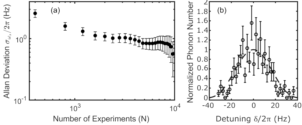
Figure 9.8: High resolution scan of an 80 MHz probe tone using the K = 12 subharmonic resonance on the axial mode. (a) An overlapped Allan deviation yields a minimum frequency uncertainty \sigma_{\omega_s}/2\pi = 0.56(32) Hz at N = 9600 . The interrogation time is fixed at \tau = 5 ms. Each individual experiment takes 22 ms and is comprised of cooling pulses, the subharmonic excitation sequence, and state detection. (b) Motional excitation spectrum generated by scanning the frequency of the probe tone. Error bars represent one standard error.
