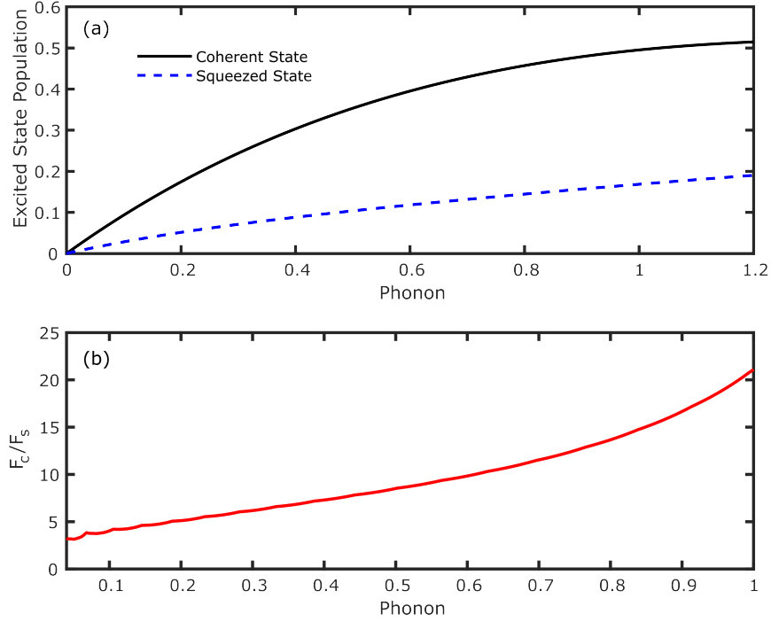
Figure 9.9: Characterizing the sensitivity of phonon readout for coherent and squeezed states. (a) The relation between population probability in excited state |^2D_{\frac{5}{2}}\rangle and phonon number for different motional states. The population is measured after applying red sideband Rabi oscillation for interrogation time \tau = \pi/\Omega_{01} , where \Omega_{01} is the Rabi frequency for the |^2S_{\frac{1}{2}}, m_J = -\frac{1}{2}, n = 0\rangle to |^2D_{\frac{5}{2}}, m_J = -\frac{5}{2}, n = 1\rangle transition. (b) The Fisher information for a coherent state ( F_c ) is greater than the Fisher information of a squeezed state ( F_s ) for any mean phonon number, making them a more desirable quantum state for precision measurements.
