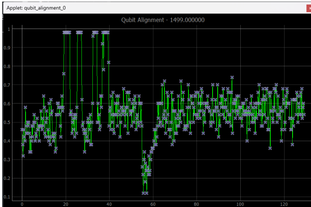
Figure 6.9: Qubit (729nm) alignment sequence.
