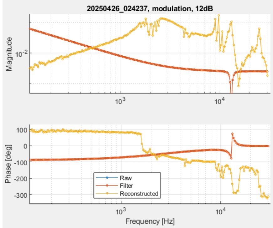
Figure 5.13: Transfer function of the 729nm filter cavity piezo feedback system. A modulation signal added to the digital servo output is demodulated at the error signal input and deconvolved from the loop filter (red) to extract the system response. The digital servo uses a PI filter with 2.8 kHz corner frequency, and a Q = 8 notch filter at 12 kHz; sharp resonances around 1 \times 10^4 Hz are further mitigated by external notch filters at 8 kHz and 13 kHz.
