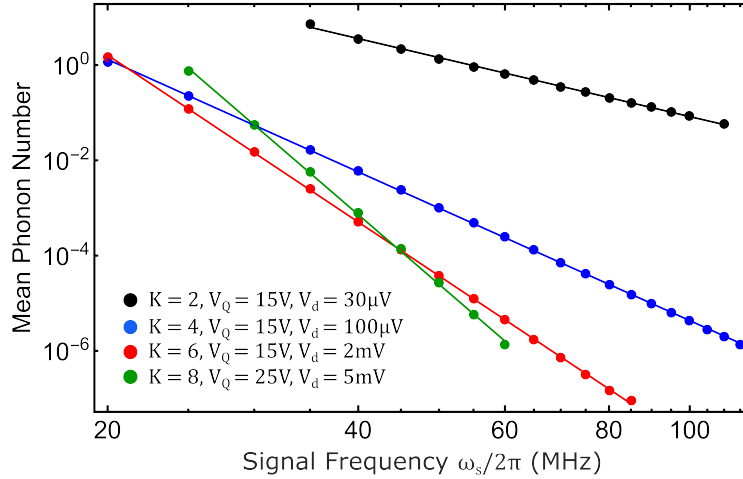
Figure 9.3: Dependence of the subharmonic excitation on the signal tone frequency \omega_s . Results are simulated using a \omega = 1 MHz secular frequency. A linear model y = mx + b is fitted to the log-log transform of the results to extract the power-law dependence at each subharmonic order. Simulated results exhibit a power-law scaling of the mean phonon number on \omega_s in good agreement with the predicted scaling of \langle n \rangle \propto \omega_s^{2K} , or equivalently, \alpha \propto 1/\omega_s^K .
