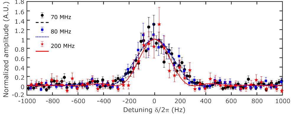
Figure 9.7: K=6 subharmonic excitation at different signal frequencies (\omega_s/2\pi)=(70, 80 \text{ and } 200 \text{ MHz}) . Lines are fits to the data using a sinc-squared profile. All data are normalized by the peak amplitudes of their fit. The interrogation time is fixed at \tau = 1.2 \text{ ms} . Error bars represent one standard error.
