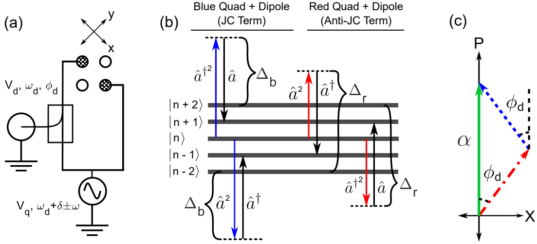
Figure 8.1: Implementation of the quantum vector signal analyzer (QVSA). (a) Schematic of the QVSA drive coupling to the quadrupole ion trap. Two quadrupole tones ( \omega_d + \delta \pm \omega ) are coupled onto the electrodes to characterize an unknown dipole tone ( \omega_d ). The dipole tone is easily supplied using either a BNC connector or a microwave horn. (b) Level diagrams for motional Raman transitions. The blue (red) arrow indicates the blue (red) quadrupole field, while the black arrow represents the dipole field. The combination of the blue quadrupole ( \omega_d + \delta + \omega ) and dipole fields results in displacement following the Jaynes-Cummings Hamiltonian (JCH) , whereas the combination of the red quadrupole ( \omega_d + \delta - \omega ) and dipole fields results in displacement according to the anti-JCH. \Delta_b = \omega_d - \omega ; \Delta_r = \omega_d + \omega ; (c) Phase space diagram showing that the phase sensitivity of the QVSA displacement \alpha arises from the interference between the displacements generated by the multiple Raman transitions; each transition is excited by one quadrupole and one dipole tone. We assume the initial phase of the quadrupole tones to be zero.
