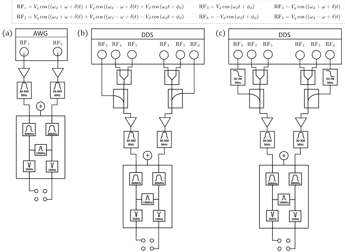
Figure 8.6: Sample RF schematic of the QVSA signal generation apparatus. (a-c) Signals are amplified (Mini-Circuits ZHL-20W-13SW+) before filtering and DC biasing (to break the radial mode degeneracy). A narrow 19 MHz band-pass filter between the QVSA electrodes shorts any pickup from the 19 MHz trap electrodes, which improves trap stability. Different combinations of filters can be used for different frequency ranges. (a) Dipole and quadrupole tones are generated with two channels of an Arbitrary Waveform Generator (Sinara “Phaser”) by setting an inter-channel phase delay of \pi and 0, respectively. (b-c) QVSA signals are generated using two banks of synchronously clocked Direct Digital Synthesis/Synthesizer (DDS) s (Sinara AD9910 Urukul). This configuration allows QVSA function as a Vector Network Analyzer (VNA) as the dipole tones can be separately passed through a Device Under Test.
