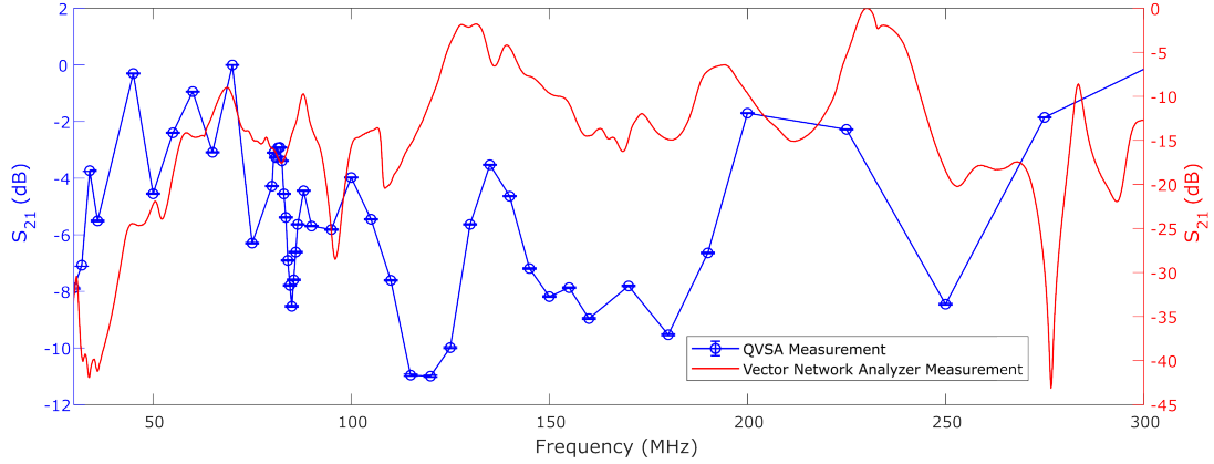
Figure 8.12: Insertion loss of the ion trap system measured using the QVSA and a commercial vector network analyzer (VNA). The wideband transfer function of a qubit control line is compared against that from a traditional measurement using a capacitor divider connected to trapping RF electrodes and a vector network analyzer over the frequency range accessible with our DDS ([20, 300] MHz). The traditional measurement fails to accurately report the filter function. Changes to the measurement conditions required to interface the network analyzer, for example impedance changes at measurement ports, likely account for this discrepancy, serving as an archetypal example of the difficulty of accurately calibrating qubit signals. Blue (red) data shows the insertion loss measured by the QVSA (VNA). Error bars for the QVSA measurements represent one standard error and are too small to be seen.
