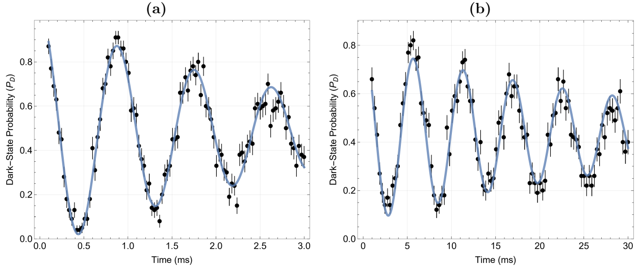
Figure 6.13: Suppression of homogeneous spin dephasing via dynamical decoupling.
