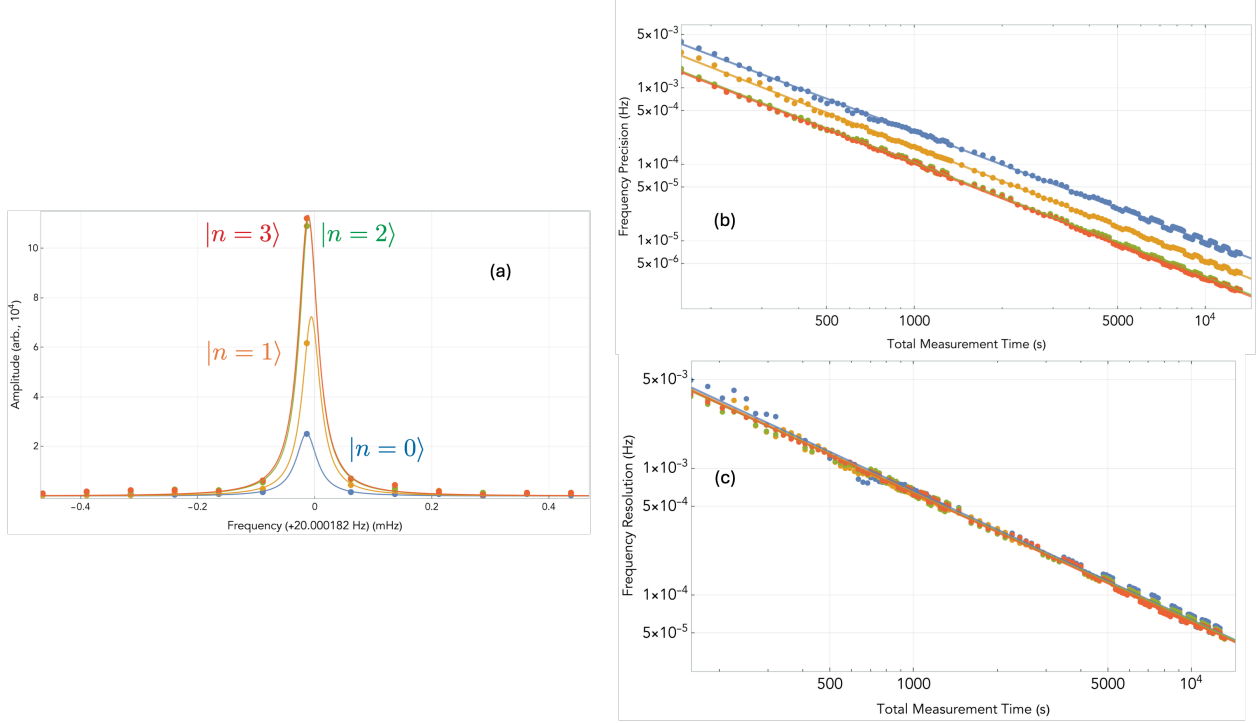
Figure 11.6: Metrological gain persists to long measurement times with Quantum-enhanced Qdyne. The displacement from an \omega_d = 86 \times 2\pi MHz dipole tone is heterodyned with a motional Raman interaction to yield an effective detuning \delta = 10 \times 2\pi Hz; this oscillation frequency is doubled in the data due to the nonlinearity of the readout procedure (see Methods). Samples are measured using a Qdyne protocol on the n = 0 (blue), n = 1 (orange), n = 2 (green), and n = 3 (red) Fock states, and use an interrogation time \tau = 300 \mu\text{s} , displacement \alpha = 0.4 , and sample period T_s = 13.3 ms. (a) FFT amplitude spectrum at total measurement time T = 1.33 \times 10^4 s. Solid curves are Lorentzian nonlinear-least-squares fits to the data. Fock state enhancement suppresses quantum noise and improves the signal-to-noise ratio (SNR), as seen in the peak amplitudes increasing with n , in agreement with the gains of Table 11.2. (b) Frequency precision \sigma_{\delta_0} of the signal peak, defined as the 95% confidence interval on the fitted Lorentzian center frequency, as a function of total measurement time T . For all n > 0 , \sigma_{\delta_0} is improved over the |n = 0\rangle case across the entire measured range of T , with no sign of the dephasing-limited deterioration in sensitivity observed in Fig. 11.5(b). Dashed lines are linear fits to the log-transformed data, yielding scaling exponents of -1.48(1) , -1.50(1) , -1.50(1) , and -1.50(1) for n = 0, 1, 2, 3 , respectively, and in good agreement with the predicted T^{-3/2} precision scaling expected for Qdyne [Bos+17, Sch+17]. (c) Frequency resolution, defined as the linewidth of the fitted Lorentzian, as a function of T . Dashed lines are linear fits to the log-transformed data, yielding scaling exponents of -1.03(1) , -1.01(1) , -1.00(1) , and -1.00(1) for n = 0, 1, 2, 3 , respectively, in excellent agreement with the well-established T^{-1} scaling expected from Fourier analysis. The achieved resolutions are Fourier-limited as Fock state enhancement does not accelerate the underlying dynamics and thus cannot improve spectral resolution. Fast oscillations in (b,c) result from spectral leakage tied to the FFT bin times; as the same bin times are used for every measurement trend, the oscillations appear synchronized.
