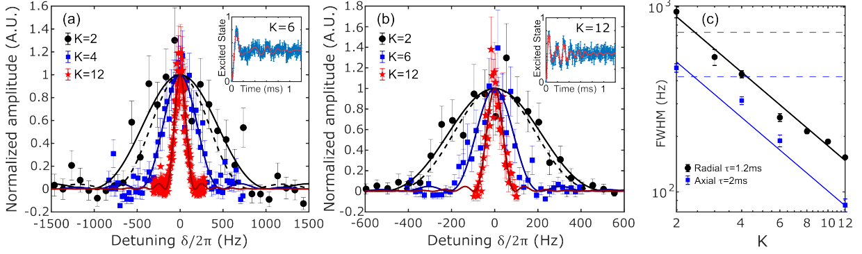
Figure 9.5: Linewidth narrowing beyond the linear Standard Quantum Limit (SQL) using subharmonic excitation. (a, b) Detection of an “unknown” signal with subharmonic excitation at \omega_s/2\pi = 70 MHz on the radial mode (a) and \omega_s/2\pi = 80 MHz on the axial mode (b). The “unknown” frequency is determined by scanning the probe detuning to maximizing the signal amplitude. For visibility, fit amplitudes are normalized to unity, with corresponding data rescaled by the same factor. Solid lines are fits of the data to a sinc-squared lineshape. Insets in (a, b): Blue sideband Rabi oscillations characterize the motional state after subharmonic excitation. Solid red lines are fits assuming a motional coherent state. (c) Dependence of linewidth on subharmonic order K . The linewidth is defined as the Full-Width at Half-Maximum (FWHM). The solid line is a linear fit to the data with no offset. (a, black data in c) An effective interrogation time is \tau = 1.2 ms used at different values of K . (b, blue data in c) \tau = 2.0 ms at different values of K . \tau is the pulse width of a square pulse of equivalent amplitude and area. (a, b, c) Dashed lines show the Fourier Transform Limit (FTL) of the applied tapered-cosine pulse envelope and corresponds to the linear SQL. Error bars represent one standard error.
