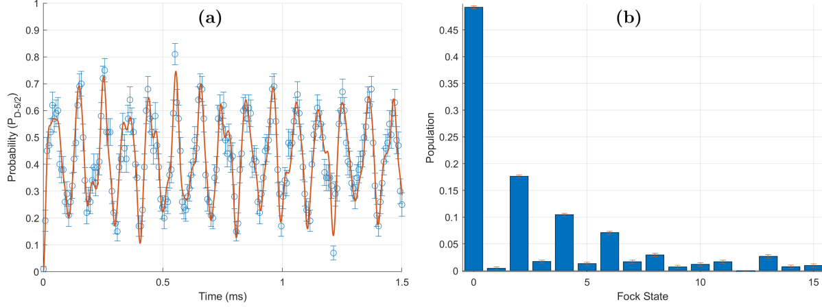
Figure 3.3: Blue Sideband Rabi oscillations (a) and Fock-state Decomposition (b) of a squeezed state |\xi| = 1.32(3) . See section 3.5.2 for a protocol overview.
