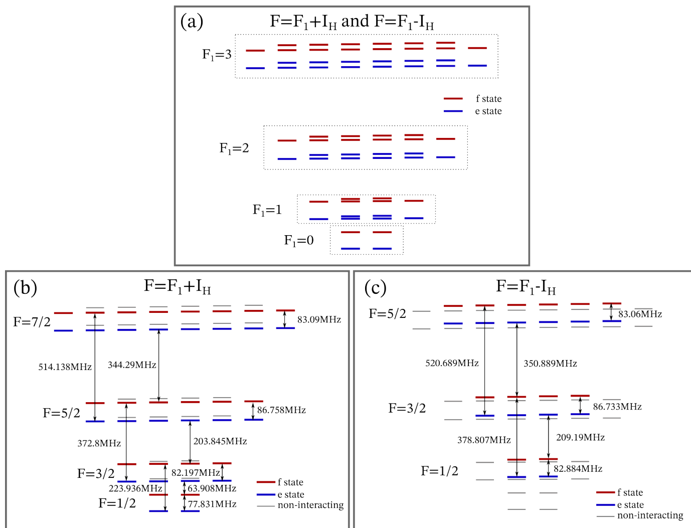
Figure 7.3: Energy level diagram for the ground state ( X\ ^2\Pi_{J=3/2} ) of \text{H}^{35}\text{Cl}^+ . (a) The J = 3/2 ground rotational level splits into hyperfine manifolds F = 3, 2, 1, 0 , formed from F_1 = J + I_{\text{Cl}} with the I_{\text{Cl}} = 3/2 chlorine nuclear spin, and further resolved into Zeeman sublevels by a B = 3.631\,97(2) G bias field. Each level is split by lambda-doubling into opposite-parity e , f states. (b, c) The weakly coupled I_{\text{H}} = 1/2 hydrogen spin partitions the structure into two non-interacting (via E1 transition) “super-hyperfine” manifolds ( F = F_1 \pm 1/2 ). The molecule is initialized into either manifold upon loading; transitions between manifolds (b) and (c) requires an M1 transition and is inaccessible with EGGS.
