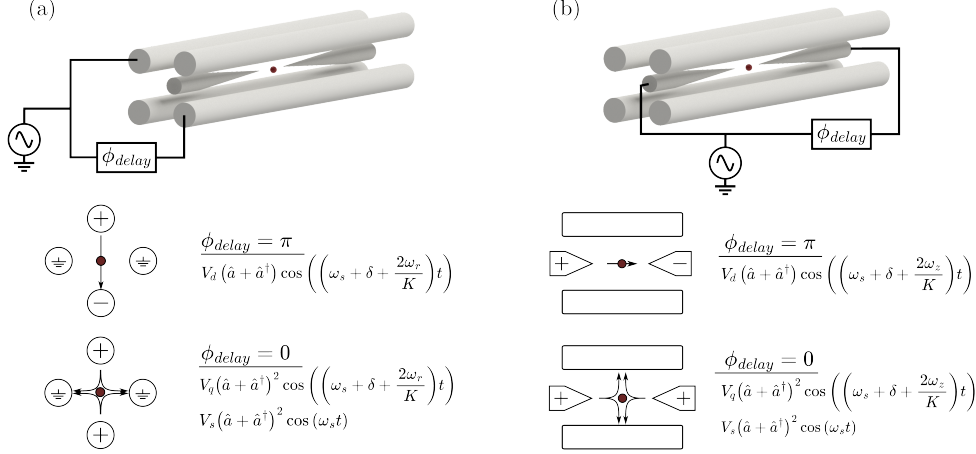
Figure 9.1: Implementation of subharmonic excitation on the radial and axial modes. (a) Subharmonic excitation is applied to excite the radial motional mode by coupling an oscillating voltage onto a pair of opposing trap electrodes. (b) The axial motional mode can be excited by instead coupling the voltage onto the axial endcaps of the trap. A dipole field is generated for a relative phase \phi_{\text{delay}} = \pi between the voltages coupled to the electrodes, while a quadrupole field is generated if the coupled voltages are exactly in phase (i.e. \phi_{\text{delay}} = 0 ).
