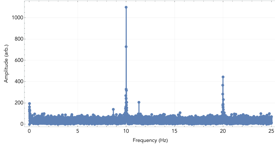
Figure 11.2: (a) Wideband synchronized readout of a GHz-band signal using motional Raman. FFT amplitude spectrum of a signal at \omega_d = 2\pi \times 1050 MHz, heterodyned by the motional Raman interaction to a detuning \delta \approx 2\pi \times 10 Hz and recovered by Qdyne without quantum enhancement (acquired with a phase-modulated quadrupole probe; see text) at a sample period T_s = 20 ms. The fundamental appears at \delta ; the peak at 2\delta is a harmonic of the nonlinear Fock state overlap readout ((11.5)). The recovered linewidth is Fourier-limited at 1/T and set by a total measurement time T = 200 s.
