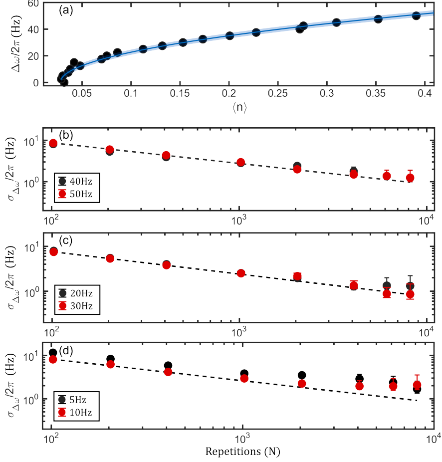
Figure 10.4: Characterizing ultimate resolution of \Delta\omega with two incoherent signal tones centered at 2\pi \cdot 86 MHz. (a) Calibration curve used to convert the measured \langle n \rangle to the parameter \Delta\omega . Experimental data are plotted as dotted points and fitted to an inversion of the analytical model (solid lines) in Eq. (10.6) with only a constant horizontal offset as the sole fit parameter. The colored band indicates the 68% prediction band. Each point is averaged over N = 5000 measurements. There is no additional rescaling. (b-d) Overlapping Allan deviations of \Delta\omega at different frequency separations \Delta\omega with fixed “known” Rabi frequency \Omega_{\text{eff}} . (b) \Delta\omega/2\pi = 40, 50 Hz. (c) \Delta\omega/2\pi = 20, 30 Hz. (d) \Delta\omega/2\pi = 5, 10 Hz. (a-d) Data was taken using a total interrogation time T = 1 ms. To simulate an incoherent signal, the relative phase between the two signal tones \Delta\phi was varied randomly between each measurement from a uniform distribution on [0, 2\pi) . Error bars represent one standard error. The dashed lines represent a 1/\sqrt{N} trend. Each repetition takes \approx 13 ms.
