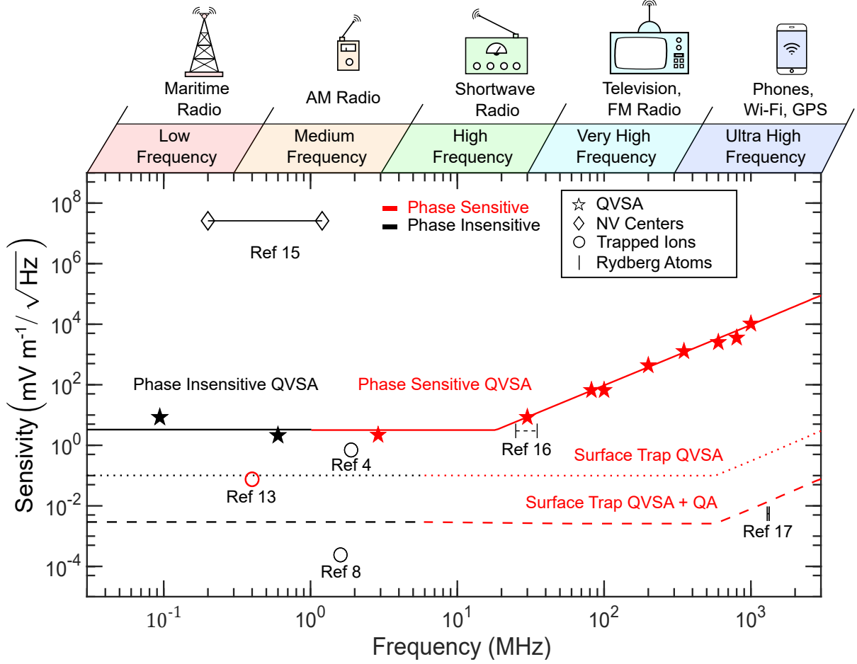
Figure 8.9: Comparisons of electric field sensitivity between different quantum sensing techniques. Phase insensitive methods are shown in black; phase sensitive methods are shown in red; \diamond : NV centers; \circ : ions; | : Rydberg atoms; \star : our measurement. The length of lines corresponds to the frequency range of operation. The solid red line represents the estimated QVSA performance in our linear trap, which aligns closely with our measurements (exact measurement results are listed in Table 8.2). Quadrupole tones are applied with a constant Mathieu q -parameter of q_q \approx 0.01 to yield a nearly constant sensitivity from 100 kHz until \approx 20 MHz. Above \approx 20 MHz, practical limitations on power prevent the constant Mathieu q -parameter of q_q = 0.01 from being applied, causing the minimum achievable sensitivity to increase with frequency. The dotted red line indicates the estimated QVSA sensitivity if implemented on a surface trap with an ion-electrode distance of 40 \mu\text{m} , ^9\text{Be}^+ as a trapped ion, a secular frequency of 2\pi \cdot 6 MHz, and a maximum quadrupole power of 39.5 dBm. The dashed red line represents anticipated near-term enhanced QVSA sensitivity in a surface trap with Quantum Amplification (QA). This comparison did not account for scaling with the number of ions.
