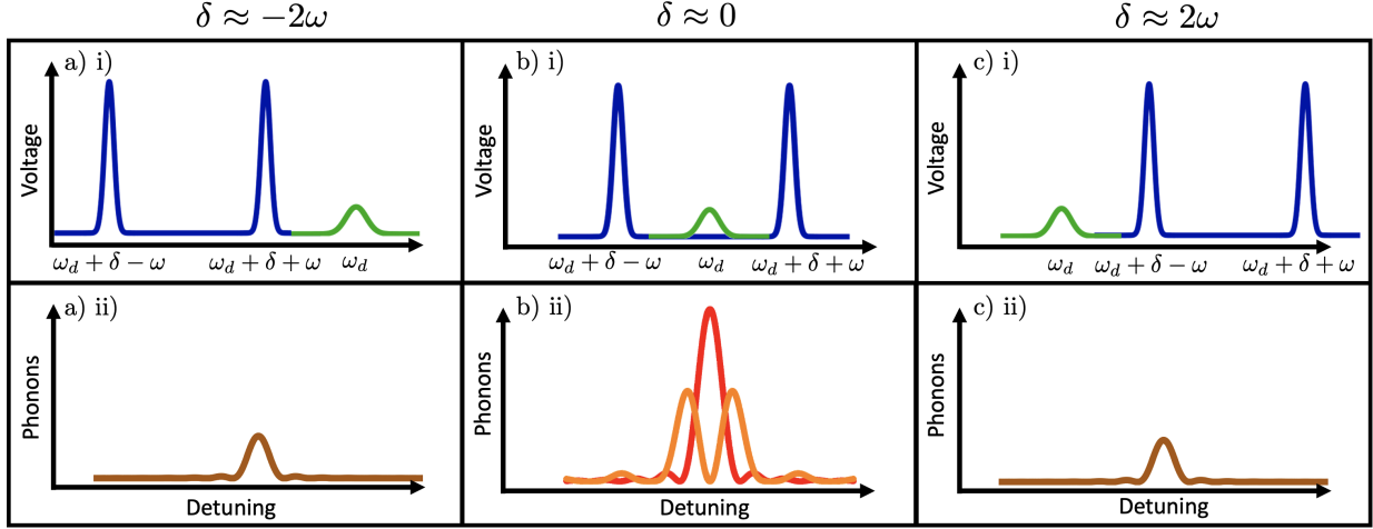
Figure 8.2: Illustration of the spectrum sweep procedure (see section 8.2.2). (a-c, i) Two quadrupole tones (blue) are swept in frequency across a weaker dipole tone (green). (a-c, ii) The resulting mean phonon number \langle n \rangle produced from the corresponding interaction in (i). (a, i-ii) The interaction is primarily determined by that between the blue quadrupole tone at \omega_d + \delta + \omega and the dipole tone at \omega_d . This interaction is phase-independent. (b, i-ii) Both quadrupole tones at \omega_d + \delta \pm \omega interact with the dipole tone at \omega_d . The resulting interaction is phase-dependent, and can produce a resonance (red) when the phase relation satisfies \phi_d - \phi_+ = 0 , where \phi_+ = \frac{\phi_b + \phi_r}{2} , or an antiresonance (orange) when \phi_d - \phi_+ = \frac{\pi}{2} . (c, i-ii) Conversely to (a), the interaction is primarily determined by that between the red quadrupole tone at \omega_d + \delta - \omega and the dipole tone at \omega_d , and is phase-independent.
