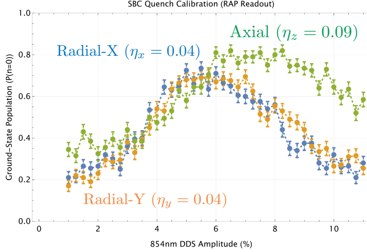
Figure 4.9: Optimization of the 854nm quench for Sideband Cooling (SBC).
