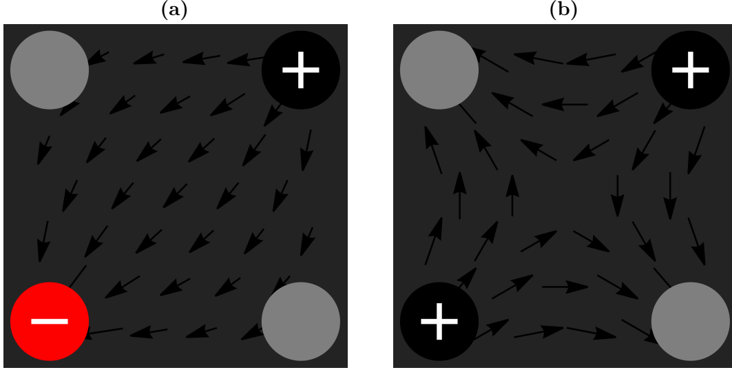
Figure 7.4: Generation of electric field gradients for molecular ion quantum logic.
