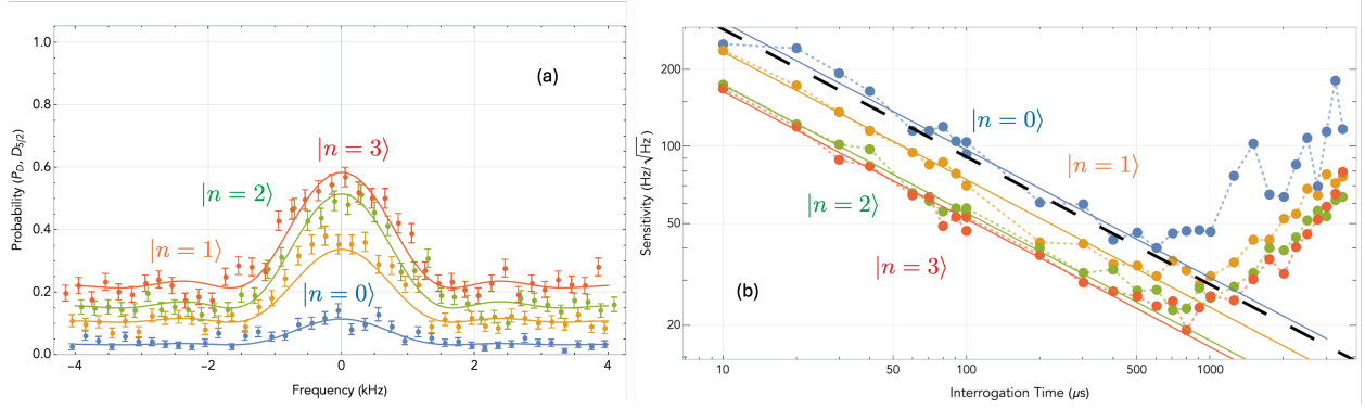
Figure 11.5: Sensitivity with conventional, quantum-enhanced spectroscopy is dephasing-limited. Colors denote use of the n = 0 (blue), n = 1 (orange), n = 2 (green), and n = 3 (red) Fock states. (a) A Rabi lineshape at \tau = 600 \mu\text{s} shows the state overlap P_n as a function of the signal detuning \delta from a motional Raman resonance at \omega_d = 86 \times 2\pi \text{ MHz} . The contrast and baseline scale with n as in Fig. 11.4(a). Solid curves are nonlinear-least-squares fits to the data using the expected form P_n = C + A e^{-|\alpha|^2} L_n^0(|\alpha|^2)^2 (see Methods) where \alpha = \alpha_{\max} \text{sinc}((\delta - \delta_0)\tau) . A , C , and \delta_0 are free parameters; \alpha_{\max} = 0.293 is fixed by calibration. Error bars represent the 1\sigma uncertainty; N = 250 repetitions are performed at each point. (b) Frequency sensitivity \delta_{\min}(\tau) = \sqrt{\tau/F_\delta} as a function of interrogation time \tau , at fixed displacement \alpha = 0.4 . For each \tau , a Rabi lineshape is acquired as in (a) (40 detuning points, N = 200 repetitions per point) and the maximum Fisher information F_\delta is extracted numerically from the smoothed fit. Solid lines are linear fits to the log-transformed data for \tau \leq 1000 \mu\text{s} ; the dashed black line is the ideal n = 0 (SQL) sensitivity \delta_{\min} = (k/\alpha\sqrt{\tau})/\sqrt{4(2n+1)} with k = 0.73 (a fixed constant for a Rabi protocol [Wu+25b]). Trends for all Fock states follow the expected \tau^{-1/2} scaling at short \tau , with sensitivities improving over |n = 0\rangle by 2.3(4) dB, 4.9(5) dB, and 5.4(4) dB for n = 1, 2, 3 respectively, in agreement with Table 11.2. At \tau \gtrsim 1000 \mu\text{s} , dephasing becomes significant and the sensitivity deteriorates, limiting the interrogation time to \tau \sim T_2 . Qdyne lifts this limit by rendering successive measurements mutually coherent, such that \tau in \delta_{\min} is substituted by the total measurement time T — this can be made arbitrarily long, limited only by the reference clock stability.
