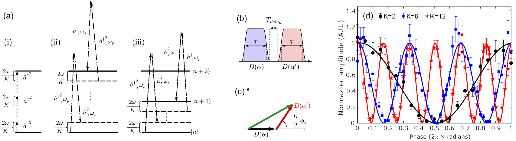
Figure 9.4: Energy-level diagrams for motional subharmonic excitation and verification via motional Ramsey spectroscopy. (a) Level diagrams for a K th-order parametric excitation (i), quadrupole subharmonic Raman excitation (ii) and quadrupole/dipole subharmonic Raman excitation (iii). (b-d) Experimental verification of accelerated dynamics via a motional Ramsey sequence with a higher-order subharmonic excitation. (b) Simplified pulse sequence of the motional Ramsey scheme used to examine the phase response. A subharmonic excitation pulse is applied for interrogation time \tau to generate a displacement \hat{D}(\alpha) . Following free evolution for time T_{\text{delay}} , a second subharmonic excitation pulse of equal area is applied with phase \phi_s relative to the initial pulse to generate a second displacement \hat{D}(\alpha') , mapping the phase onto the ion's motional state. (c) Motional Ramsey protocol in phase space. The phase \phi_s rotates the second displacement \hat{D}(\alpha') relative to the first. The phase dependence at order K thus corresponds to the periodicity of the Ramsey fringes. (d) Ramsey fringes generated by scanning the phase \phi_s of the second subharmonic excitation pulse at different orders K . Here, \tau = 1 ms with delay time is T_{\text{delay}} = 50 \mu\text{s} . Solid lines are fits of the data to a sine. Excitation amplitudes for all subharmonic orders K are normalized for comparison. Error bars represent one standard error.
