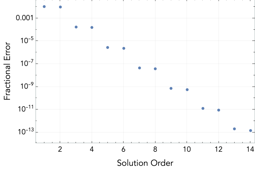
Figure 2.3: Fractional error of higher-order solutions for the secular frequency \beta .
