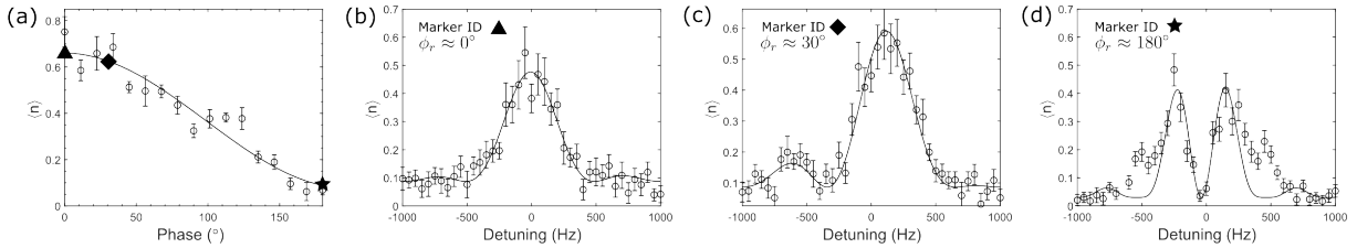
Figure 8.3: Phase dependence of the spectrum sweep procedure. The phase relation between the QVSA tones fundamentally changes the lineshape of the resonance. By sweeping just \phi_r , the phase dependence is reduced to \langle n \rangle \propto \cos^2(\frac{\phi_r}{2}) . (a) shows a phase sweep at the resonance (i.e. \delta = 0 ), with three characteristic phases marked by a triangle (b), a diamond (c), and a star (d). Voltage parameters vary between marked points. (d) illustrates the production of an antiresonance, which occurs when the red sideband is completely out of phase with the blue sideband (see Figure 8.1(c) for a graphical representation). The amplitude discrepancy between (a) and (b-d) is due to a difference in the applied QVSA voltages. Error bars represent one standard error. The solid lines are fitted lines using eq. (8.9).
