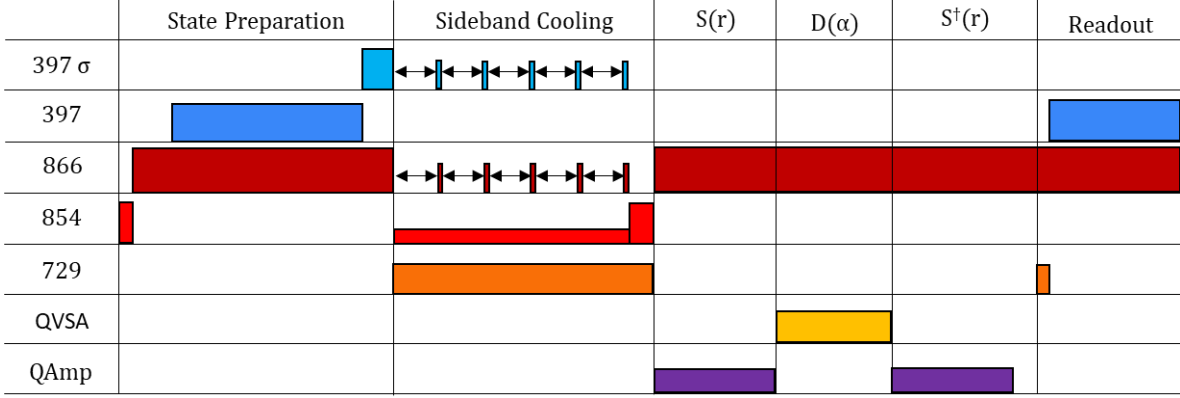
Figure 8.5: Pulse sequence for the QVSA with Quantum Amplification. The ion is Doppler cooled and optically pumped into the |^2S_{1/2}, m_J = -\frac{1}{2}\rangle state. Continuous sideband cooling subsequently prepares the ion near the ground motional state |n = 0\rangle . Quantum Amplification is achieved by preparing the ion in a squeezed state before applying the QVSA pulse, which amplifies the displacement and minimizes uncertainty along the squeezing axis. The squeezing is then reversed via an anti-squeezing pulse, returning the ion to a coherent state.
