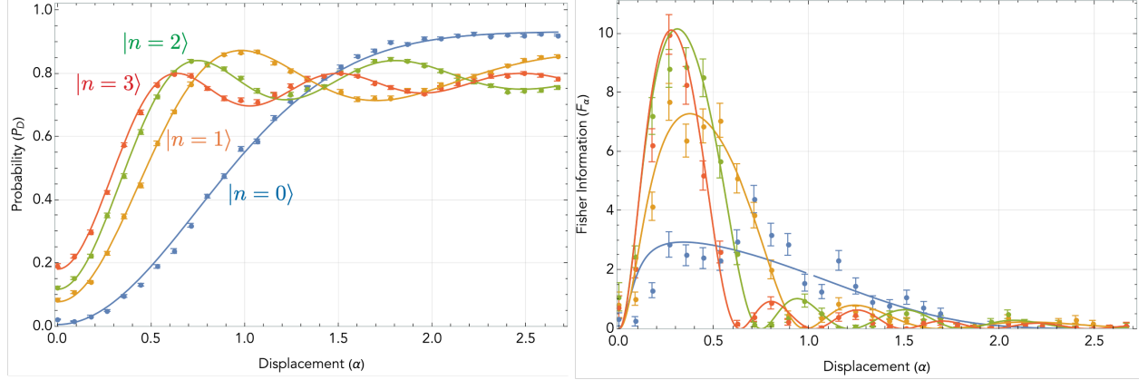
Figure 11.4: Benchmarking quantum enhancement with motional Fock states. (a) Measured state overlap P_n = |\langle n | \hat{D}(\alpha) | n \rangle|^2 as a function of the displacement amplitude \alpha , for Fock states n = 0 (blue), n = 1 (orange), n = 2 (green), and n = 3 (red). Displacements are produced via the motional Raman interaction with interrogation time swept over \tau \in (0, 100] \mu\text{s} at fixed signal amplitude. N = 5000 repetitions are taken at each point to ensure smoothness for numerical differentiation in (b); error bars represent the 1\sigma standard error and are too small to see. Solid curves are fits to the data of the form P = C + A e^{-|\dot{\alpha}\tau|^2} L_n^0(|\dot{\alpha}\tau|^2)^2 , with A , C , and \dot{\alpha} as free parameters. A and C are used to account for protocol infidelities and decoherence. Non-monotonic behavior for |n > 0\rangle reflects the negativity of the Fock state Wigner function, which allows the overlap to vanish before the states are fully separated. (b) Fisher information F_n(\alpha) = (\partial_\alpha P)^2 / (P(1 - P)) extracted numerically from the data in (a) (points), with solid curves obtained by computing F_n from the analytical fits in (a). A maximum F_{n=3} = 10.0(7) at \alpha = 0.27 represents an improvement of 4.0(3) dB beyond the SQL (Table 11.1); selected values are presented in Tables 11.2, 11.1. The |n = 0\rangle measurement yields F_0 = 4.4(5) , within 1\sigma of the SQL value of \mathfrak{F} = 4 . Discrepancies from the ideal Quantum Fisher Information \mathfrak{F}_n = 4(2n + 1) reflect the compounding of pulse errors and decoherence over the many pulses required for higher- n preparation.
