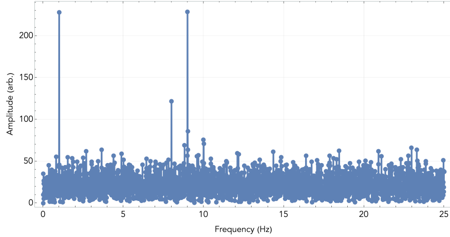
Figure 11.3: Two-tone response of synchronized readout. FFT power spectrum of two equal-amplitude dipole tones injected at detunings 2\pi \times 5 Hz and 2\pi \times -4 Hz, heterodyned by the motional Raman interaction and recovered by Qdyne at probe displacement \alpha \approx 0.4 (sample period T_s = 20 ms). As the Fock state overlap readout (eq. (11.5)) measures |\alpha|^2 , larger cross terms at 1, 9 Hz appear in addition to the expected single-tone terms at 8, 10 Hz.
