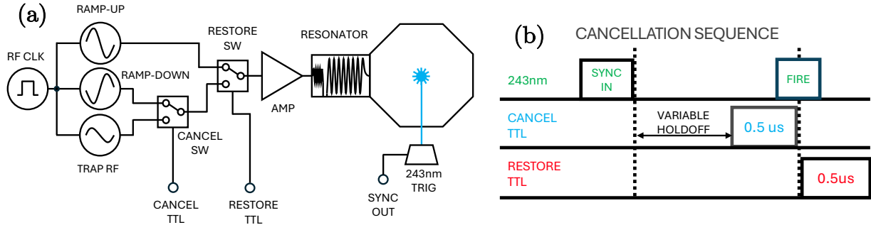
Figure 5.19: Trap RF cancellation system.
