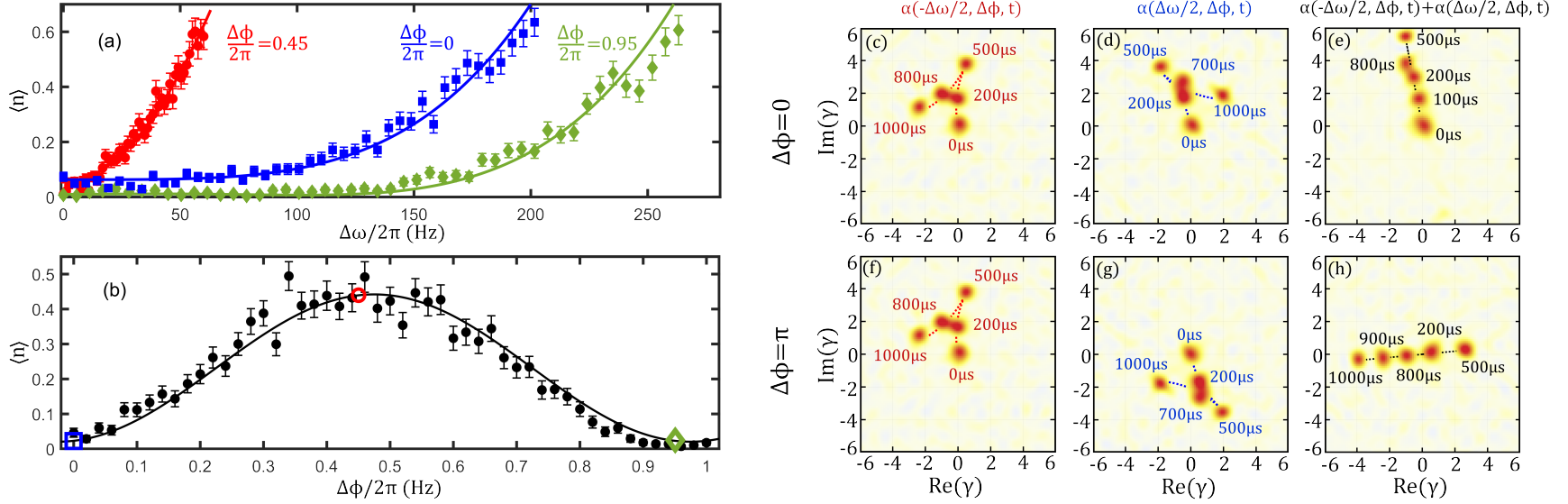
Figure 10.2: Dependence of the QFS protocol on the relative phase \Delta\phi between two signal tones \omega_1 \approx \omega_2 \approx 2\pi \cdot 86 MHz. (a) Super-resolution spectrum of \Delta\omega = \omega_2 - \omega_1 for \Delta\phi = 0.9\pi (red, circle), \Delta\phi = 1.9\pi (green, diamond), and \Delta\phi = 0 (blue, square). (b) Measured \langle n \rangle as a function of \Delta\phi at \Delta\omega/2\pi = 50 Hz. Experimental data (dotted points) are in excellent agreement with fits to eq. (10.5) (solid lines). Almost all parameters used in the fit are independently measured or controlled (e.g. \Omega_{\text{eff}} and T ), with a uniform vertical offset being the only fitting parameter. No additional vertical or horizontal scaling is applied. (a-b) A total interrogation time T = 1 ms was used. Error bars represent one standard error. Each point is averaged over N = 600 repetitions. (c-h) Phase space evolution of the QHO Wigner function under the QFS protocol for \Delta\phi = 0 (c, d, e) and \Delta\phi = \pi (f, g, h) at \Delta\omega/2\pi = 200 Hz. The Wigner function is experimentally measured using motional state tomography. The blue (red) dashed line represent the analytical phase-space trajectory due to evolution under a single tone. The black dashed lines show the resultant trajectory when both tones are applied. (e,h) Following phase reversal at T = 500\mu s , the motional trajectory retraces itself to remove the \Delta\omega -independent displacement, leaving only a \Delta\omega -dependent displacement.
